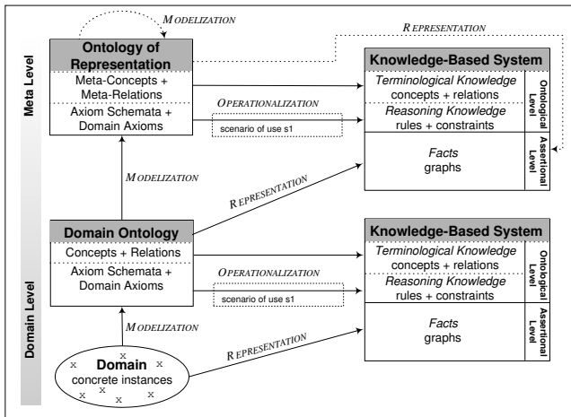
Figure 7: Overview of the interactions between Domain Ontology, Ontology of Representation and KBS.
