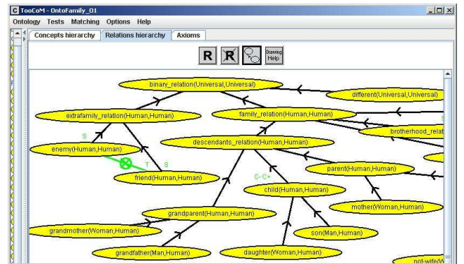
Figure 2: Representation of a relation hierarchy in OCGL. A crossed circle represents an incompatibility (or exclusivity) between two relations, algebraic properties and cardinalities of a relation are indicated by symbols above the name of the relation (S for symmetry, T for transitivity, C+ and C- for the cardinalities, etc.).
