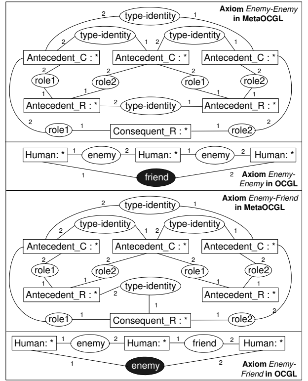
Figure 9: Two axioms represented in MetaOCGL “The enemy of my friend is my enemy” and “The enemy of my enemy is my friend”. The type_identity links denote that the nodes are of the same type in the axiom. The two graphs are the same without considering type_identity links, but they differ when considering these links, because relations in the hypothesis part of the axiom at the top have the same type ( enemy ), but not those of the axiom at the bottom ( enemy and friend ).
