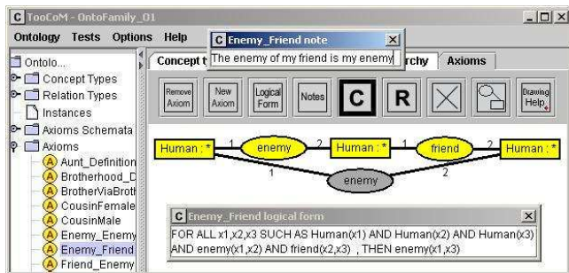
Figure 3: Representation in OCGL of the axiom “ The enemy of my friend is my enemy ”. The bright nodes represent the antecedent part, the dark ones the consequent part. The logical expression of the graph is automatically generated.
