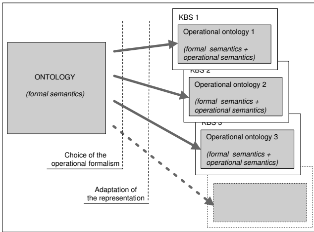
Figure 4: Operationalization process: an overview. The same ontology can lead to several operational ontologies appropriated to different KBS.
