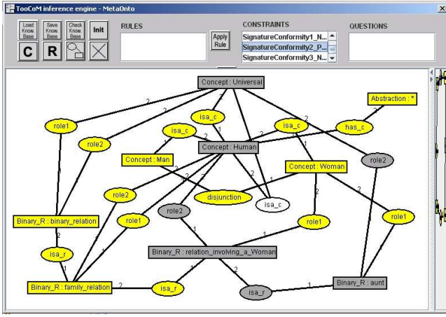
Figure 10: Operationalization of MetaOCGL for ontology verification.
