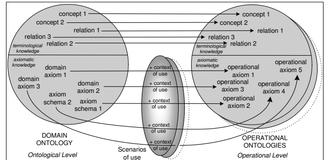
Figure 5: Operationalization process: in details. Each combination of contexts of use produces an operational ontology different from the others.
