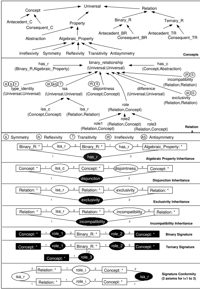
Figure 8: Concepts, relations and some of the axioms of MetaOCGL.
